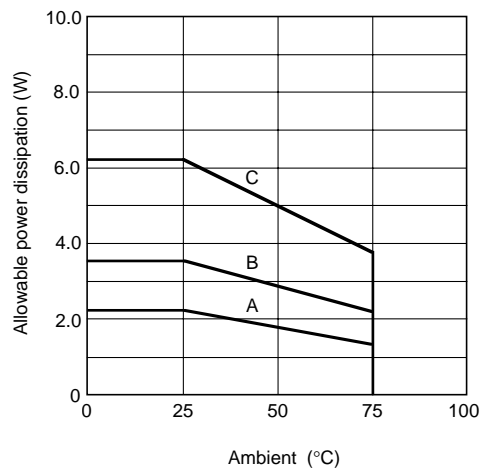
Thermal derating
